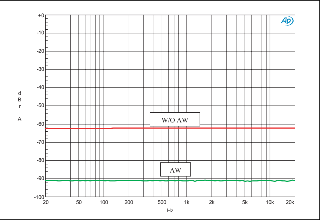
Figure 25. BTL signal-to-noise ratio at 1 W output
