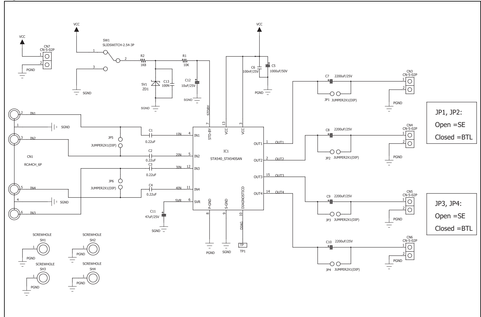
Figure 7. STEVAL-CCA040V1 schematic
