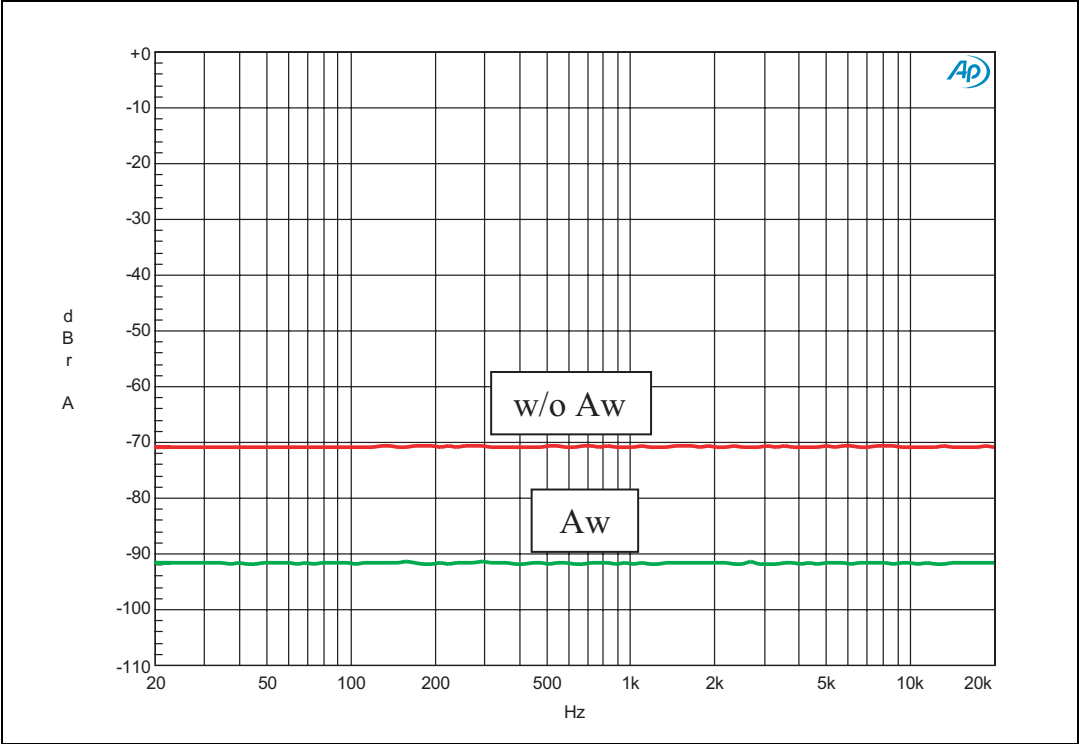
Figure 17. SE signal-to-noise ratio at 1 W output
