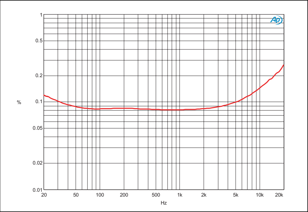
Figure 23. BTL THD vs. frequency
