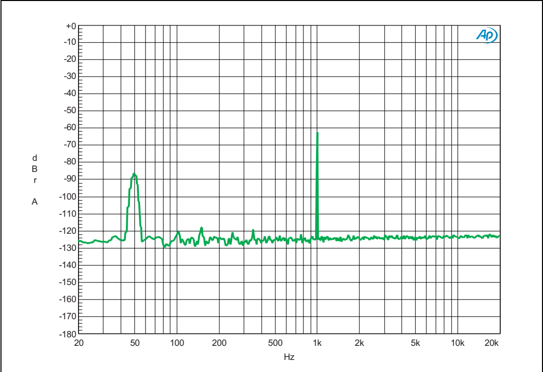
Figure 27. FFT 1 kHz, -60 dB at 1 W output
