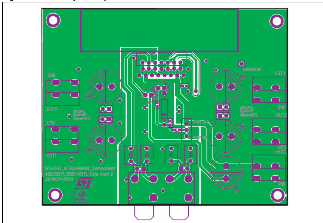
Figure 8. PCB layout - top view
