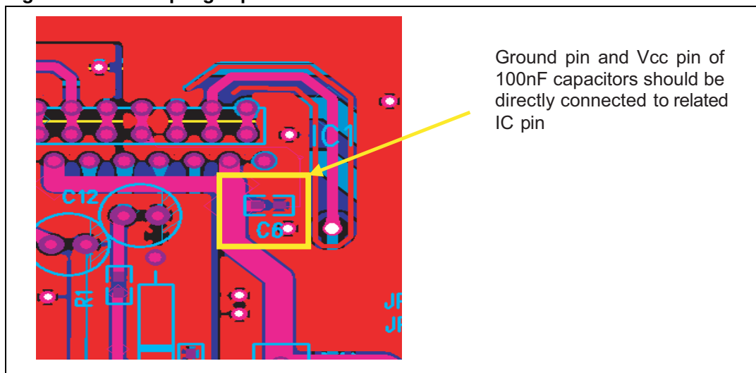
Figure 10. Decoupling capacitors
