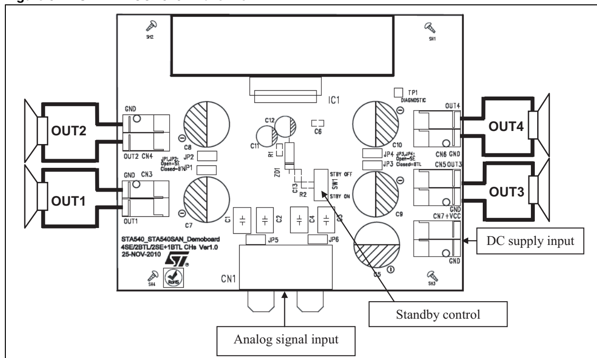
Figure 3. STEVAL-CCA040V1 overview
