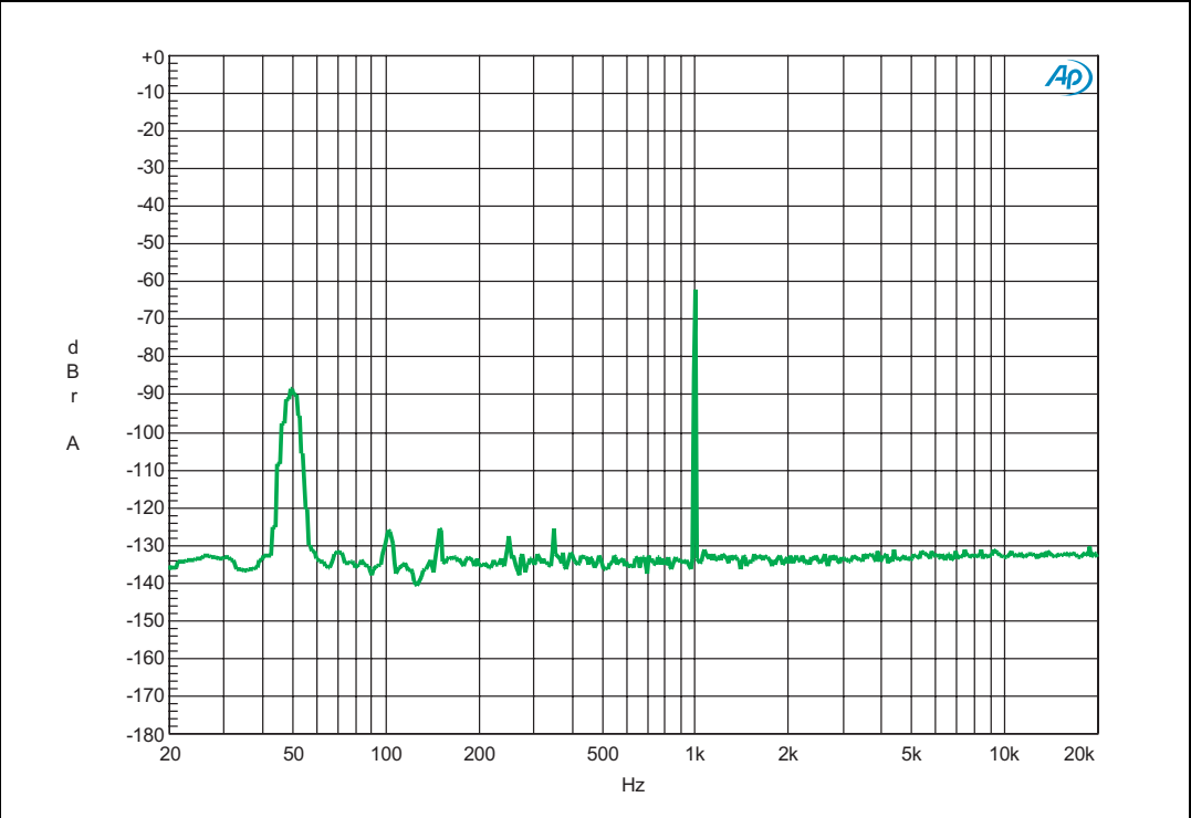
Figure 19. SE FFT 1 kHz, -60 dB at 1 W output
